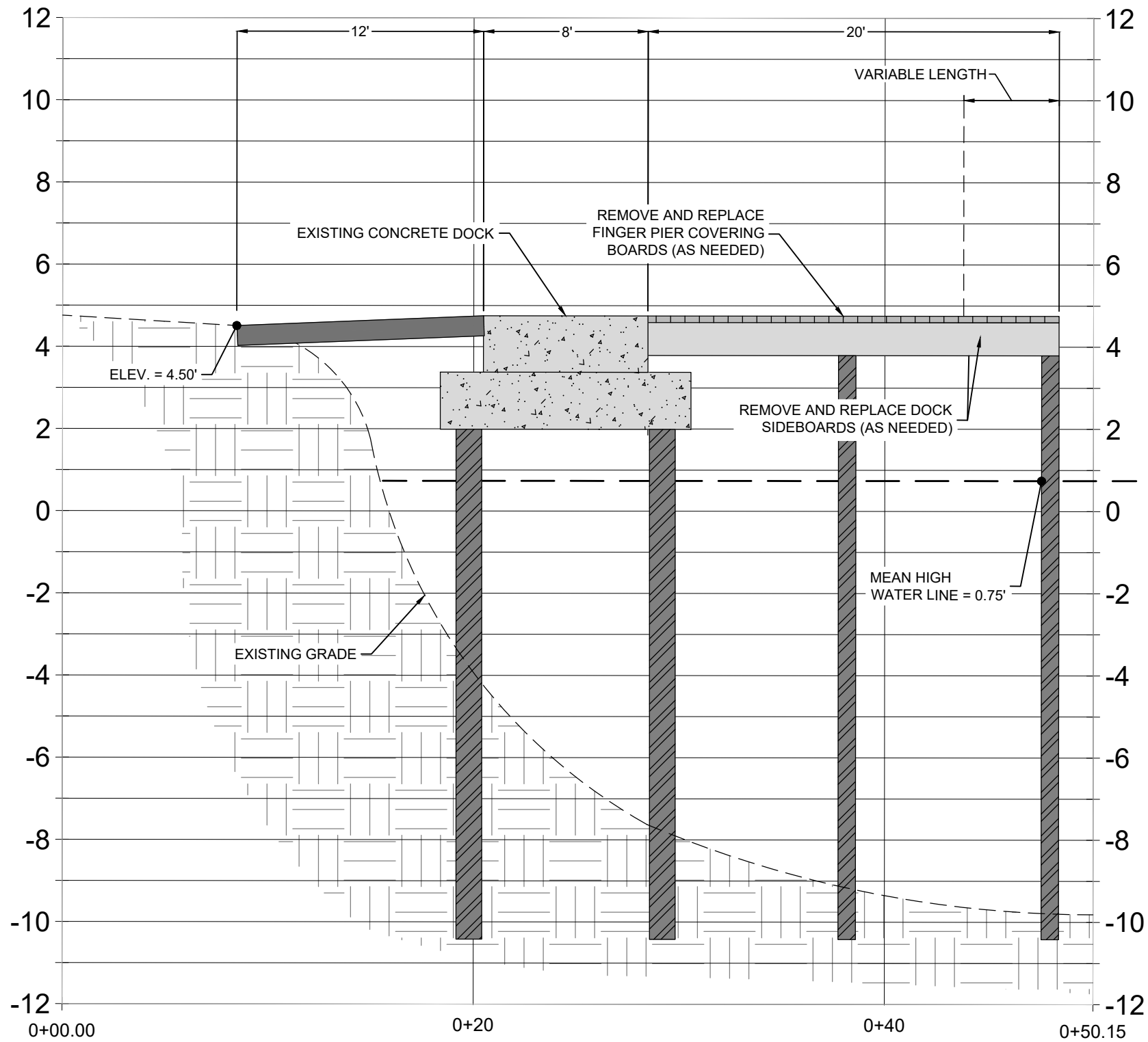
A-A C4 PROFILE A-A "DOCK REPAIR & REPLACE" SCALE: HORIZONTAL 1"=20' VERTICAL 1"=2'
